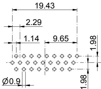
PCB Layout tolerances +/-0.1
